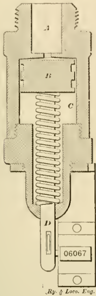
AIR PUMP STROKE COUNTER.
